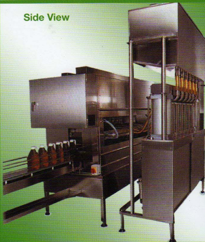
In-Line Piston Filling Machine with 8 Filling Nozzles
